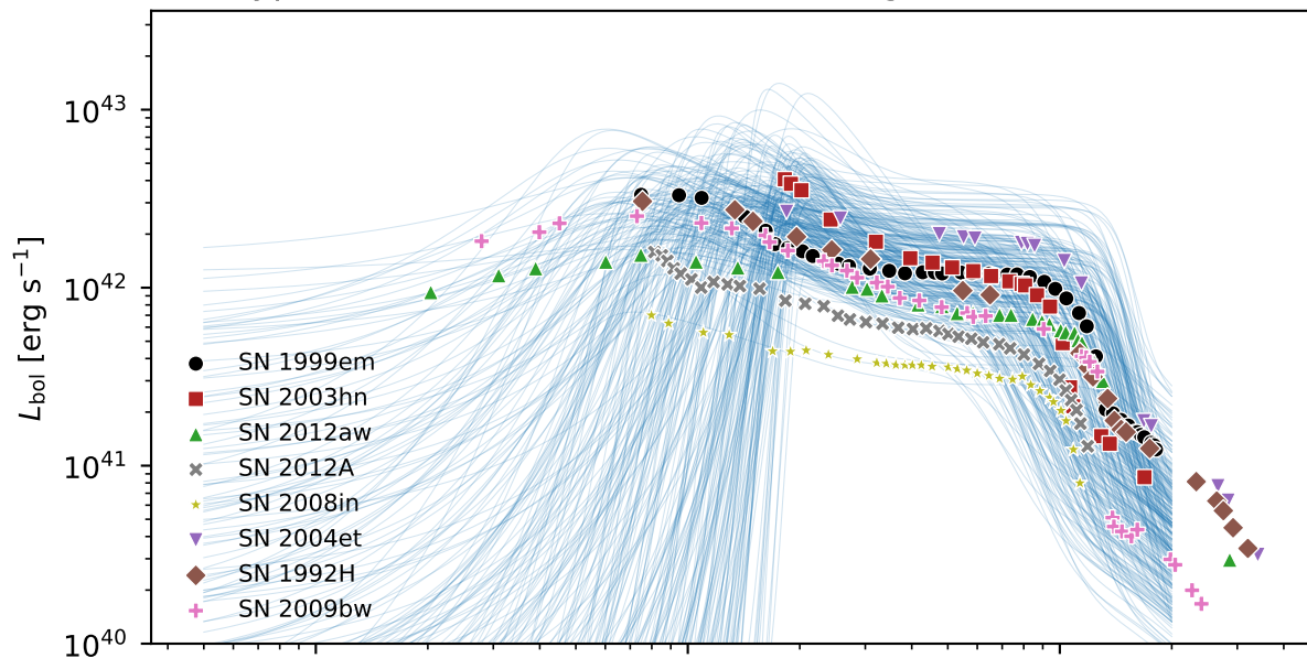
Type IIP SNe: simulated bolometric light curves (n=300)
