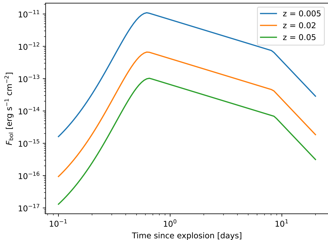
Observed bolometric flux at three redshifts
