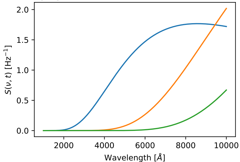
Normalized shape (integrates to 1 over \nu ) 1e-15
