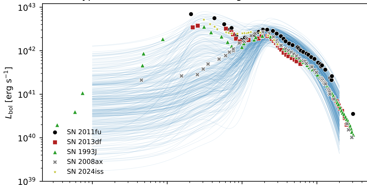
Type IIb: simulated bolometric light curves (n=300)
