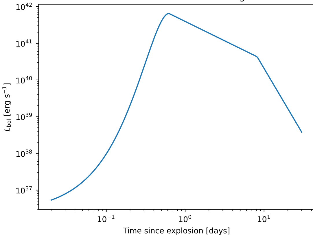
One simulated kilonova bolometric light curve
