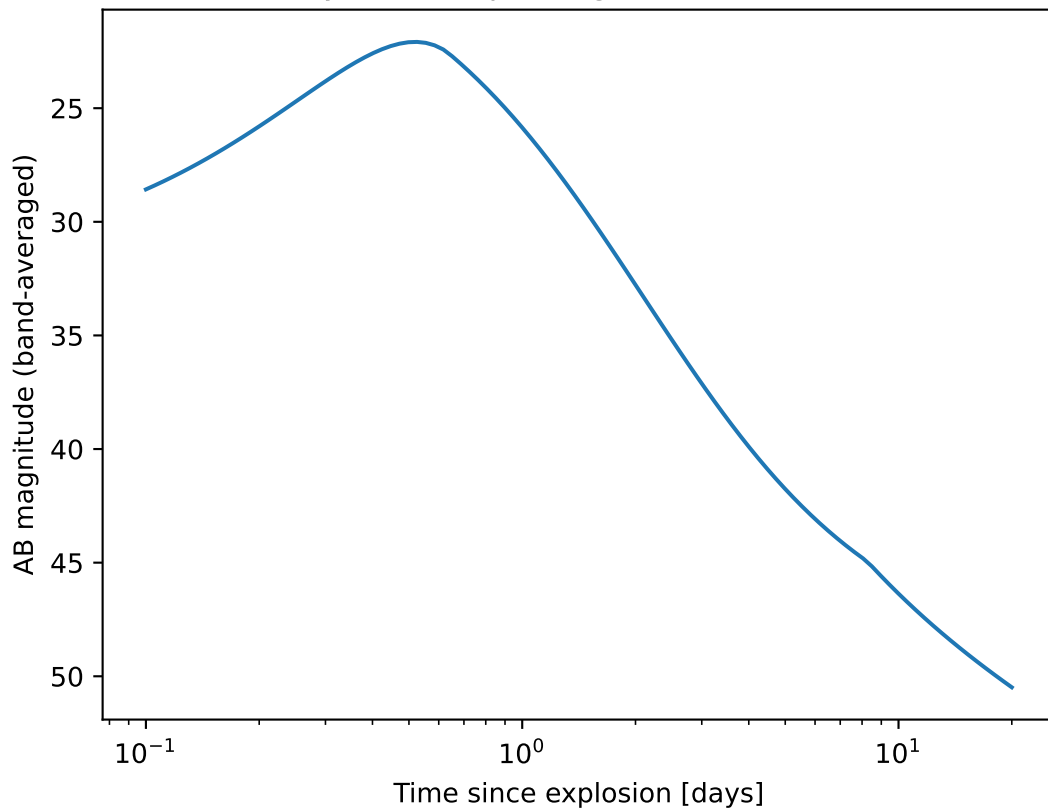
A toy UV bandpass light curve, z = 0.01
