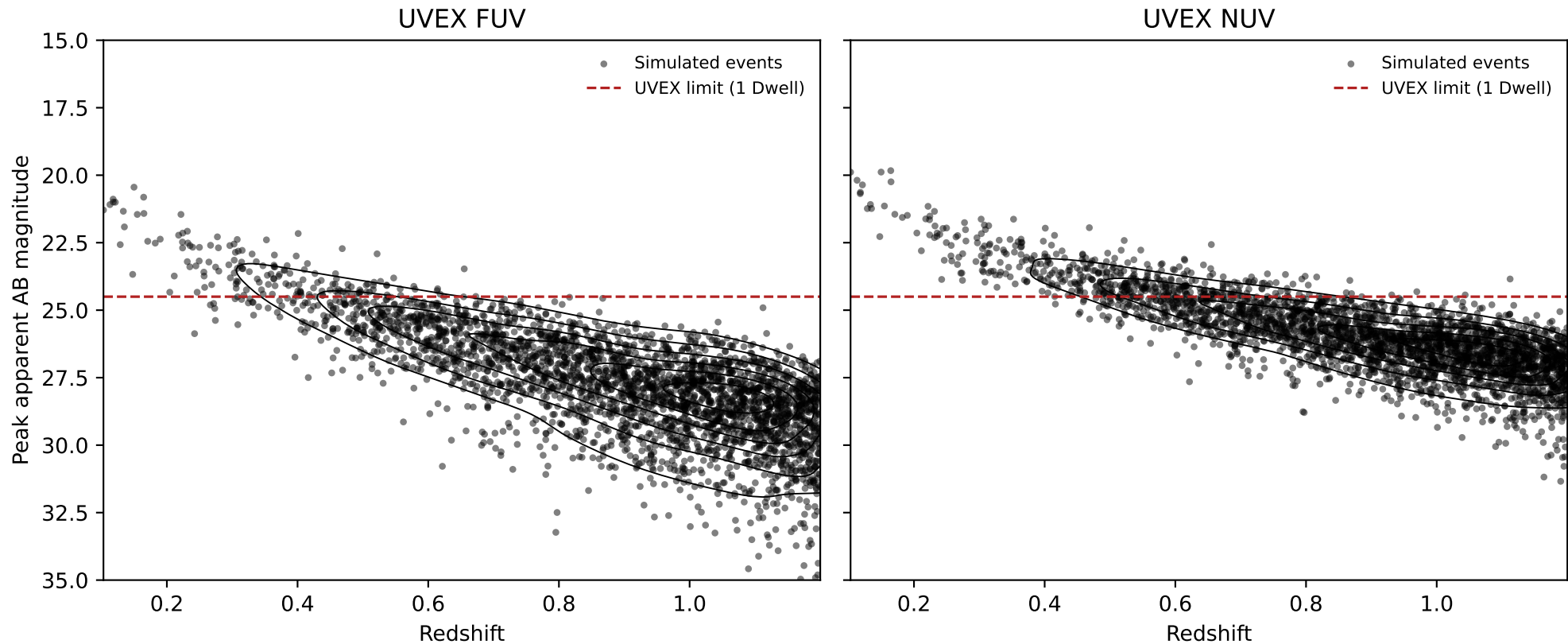
Type IIP + Excess SNe: peak apparent magnitude vs. redshift (n=3000)
