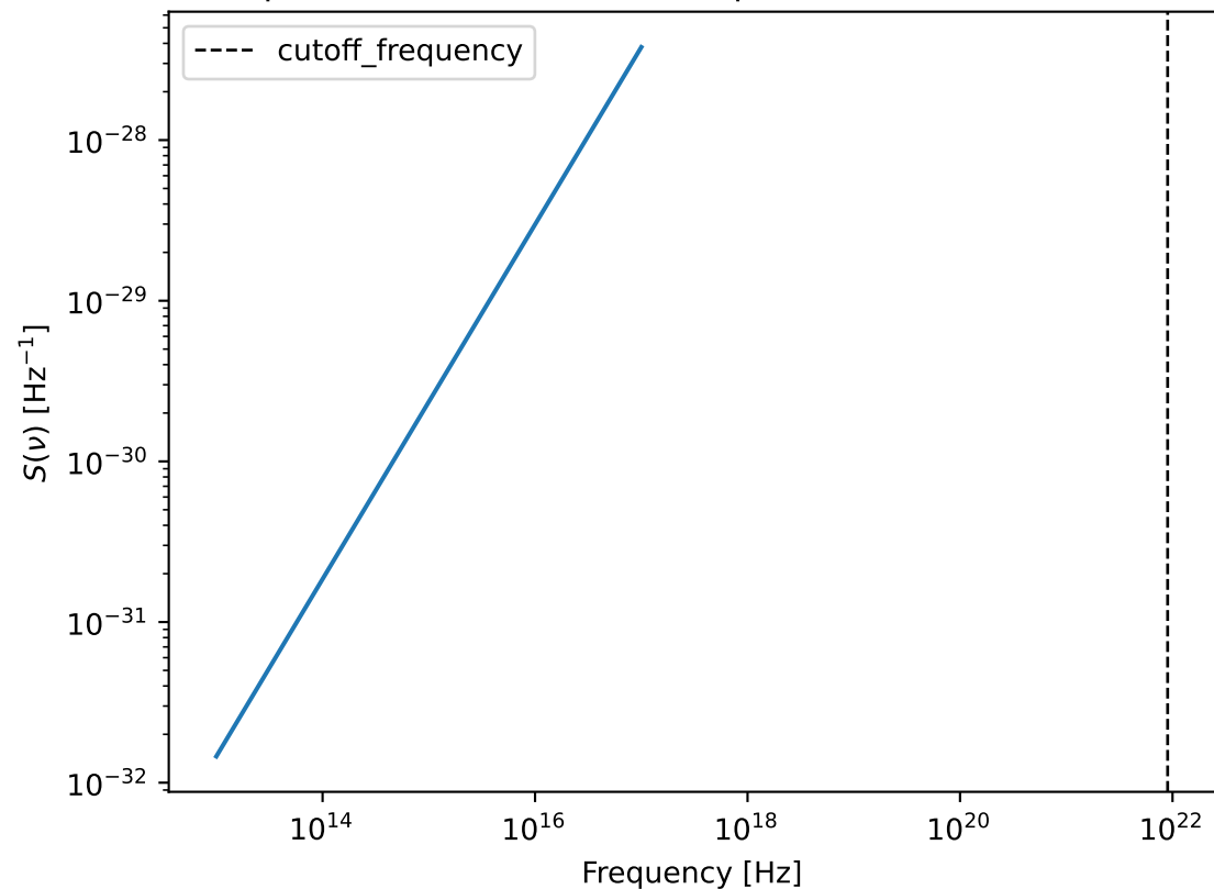
ExponentialCutoffPowerLawSpectrum, one realization
