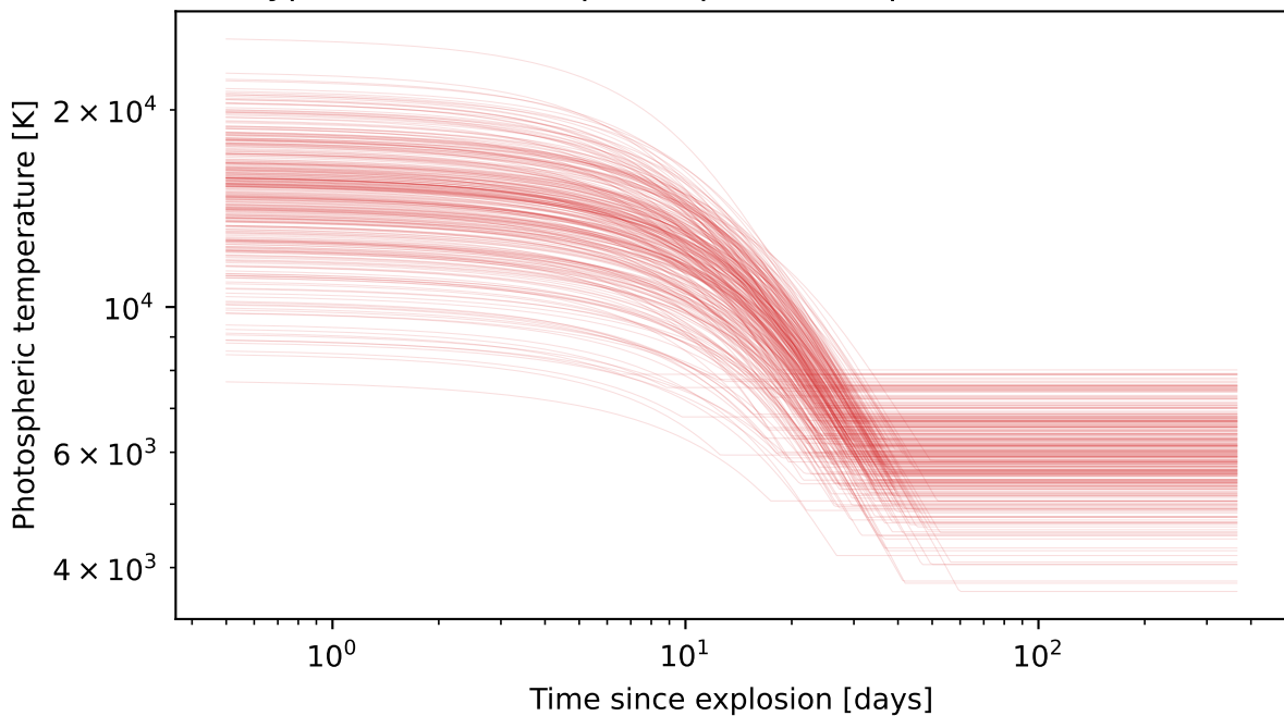
Type Ia: simulated photospheric temperatures (n=300)
