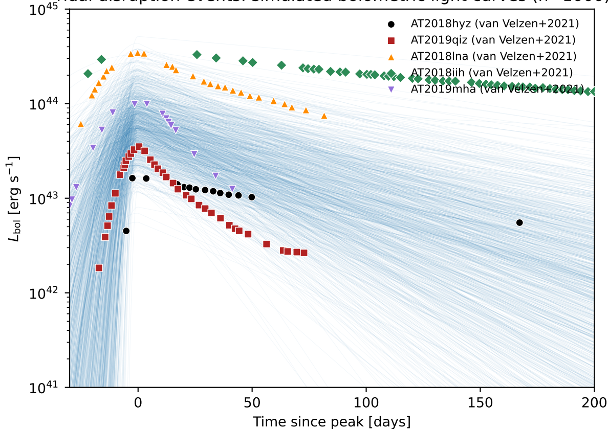
Tidal disruption events: simulated bolometric light curves (n=1000)
