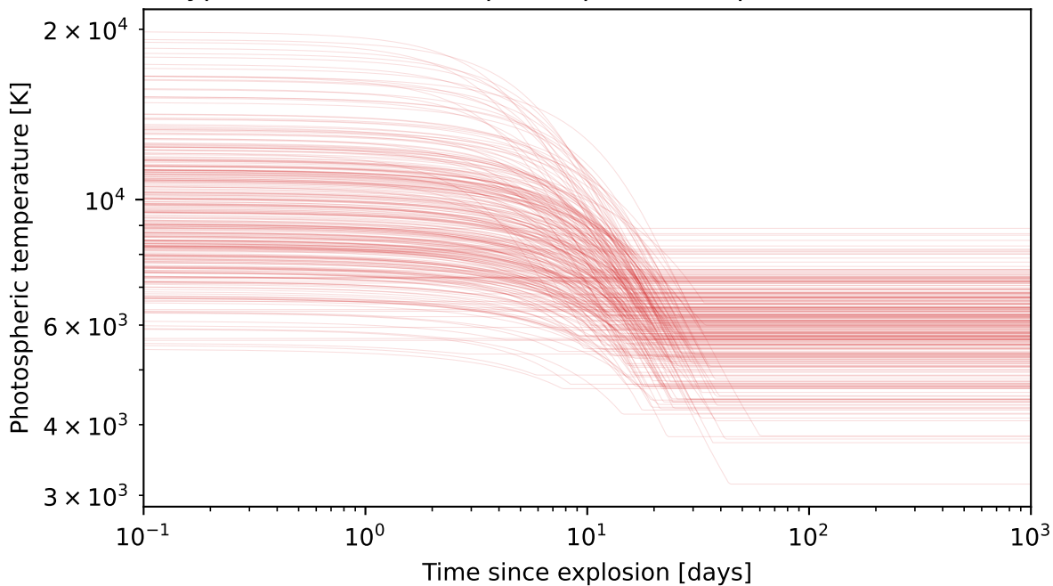
Type Ic-BL: simulated photospheric temperatures (n=300)
