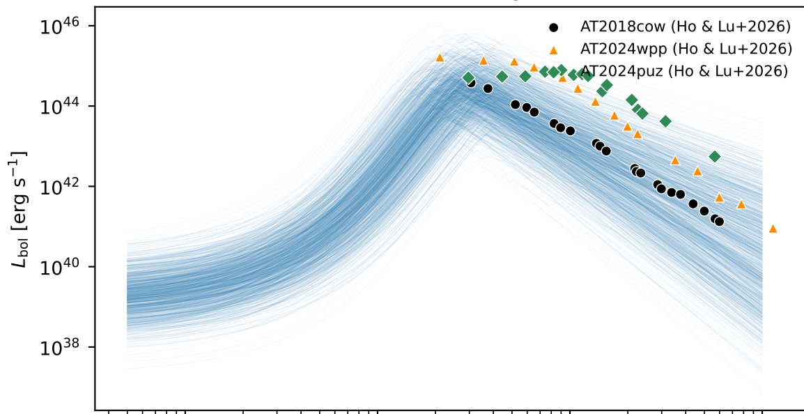
LFBOTs: simulated bolometric light curves (n=1000)
