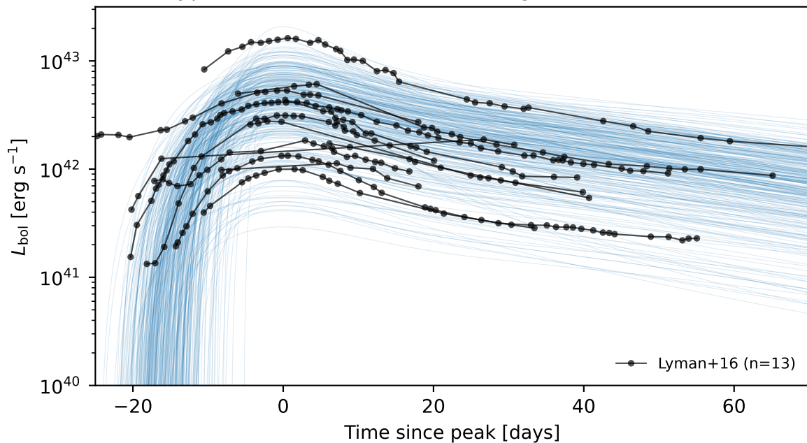
Type Ib: simulated bolometric light curves (n=300)
