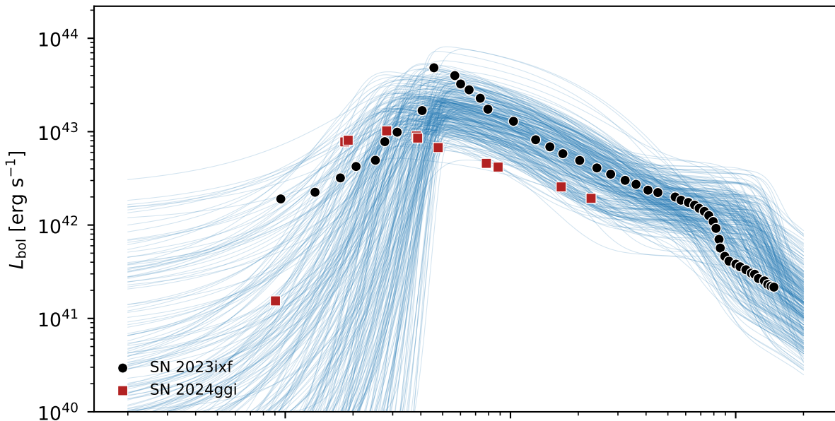
Type IIP + Excess SNe: simulated bolometric light curves (n=300)
