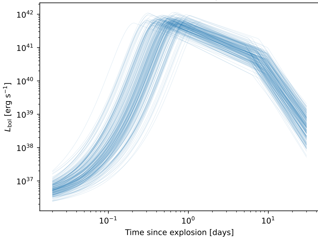
200 simulated kilonova light curves
