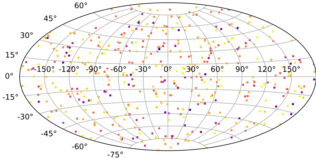
427 sampled ToyNova events, whole sky, one year
