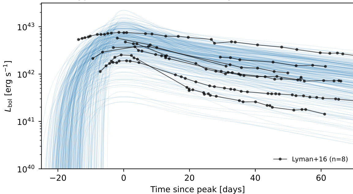
Type Ic: simulated bolometric light curves (n=300)
