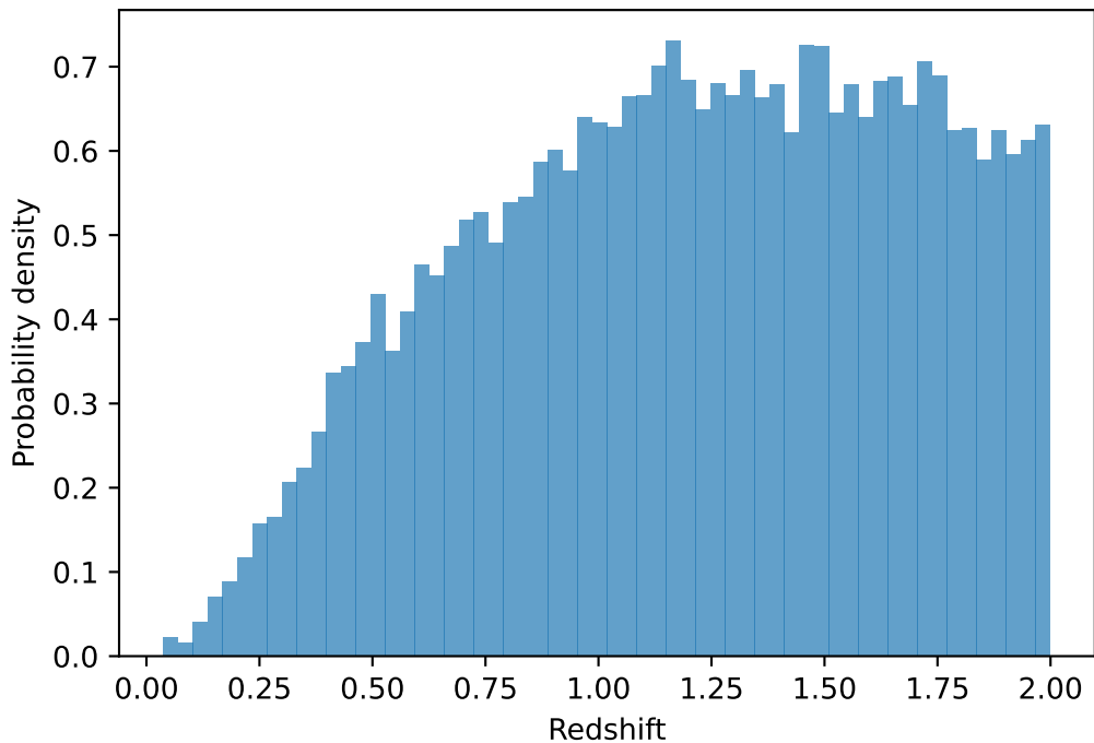
TDE redshift distribution (rate-weighted, inverse-transform sampled)
