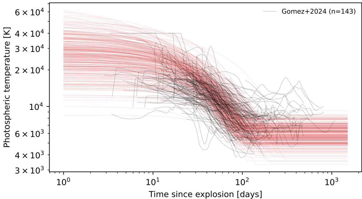
SLSN-I: simulated photospheric temperatures (n=300)
